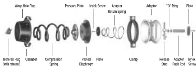
Rear Section
